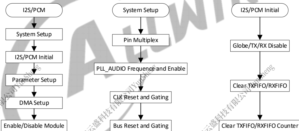
Figure 15-21 I2S/PCM Operation Flow
