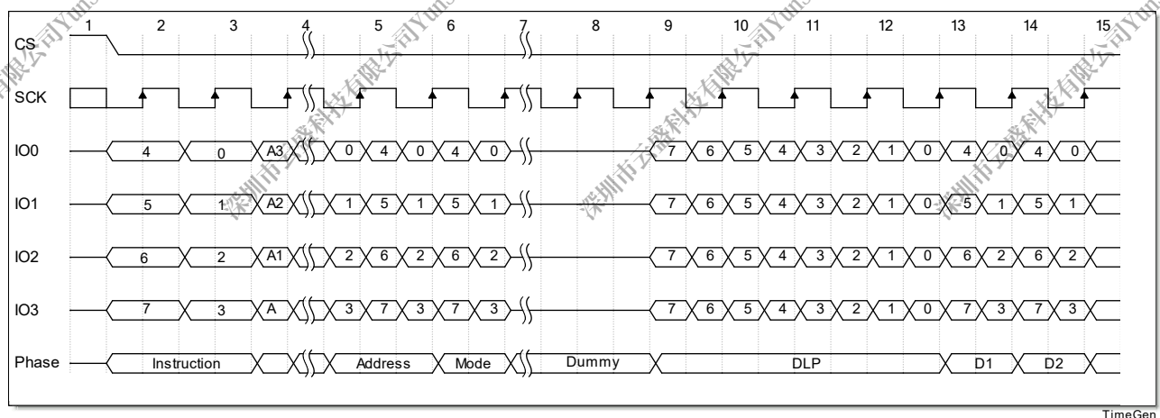
Figure 10-18 SPI DTR Transfer Example, 4-4-4
