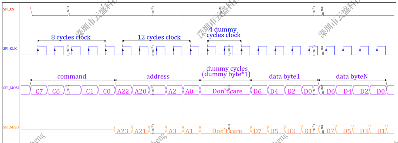
Figure 16-55 SPI Dual I/O Mode
