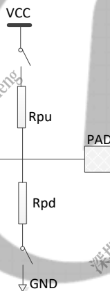
Figure 16-38 Pull-up, Pull-down, and High-impedance Input Mode
