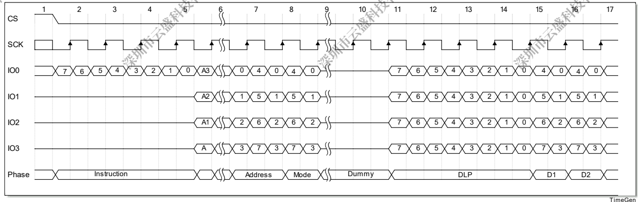
Figure 10-18 SPI DTR Transfer Example, 4-4-4
