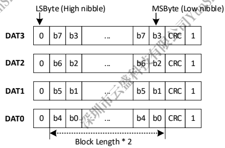
Figure 10-6 Data Packet Format for DDR
