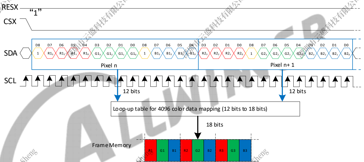
Figure 16-70 RGB444 3-Line Interface Transmit Video Format
