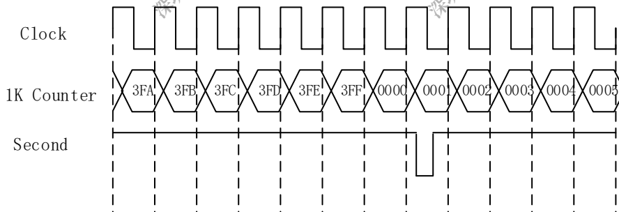
Figure 9-2 RTC Counter
