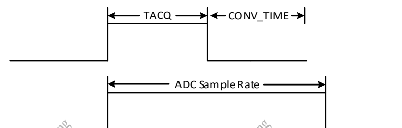
Figure 16-28 GPADC Timing Requirement
