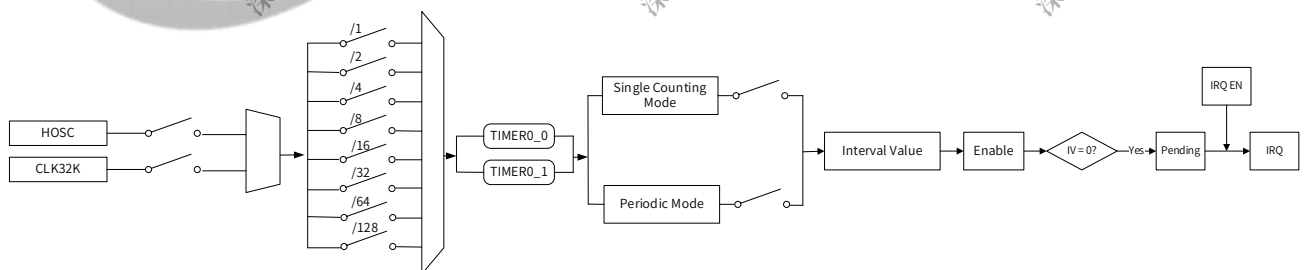
Figure 8-2 Block Diagram for the Timer
