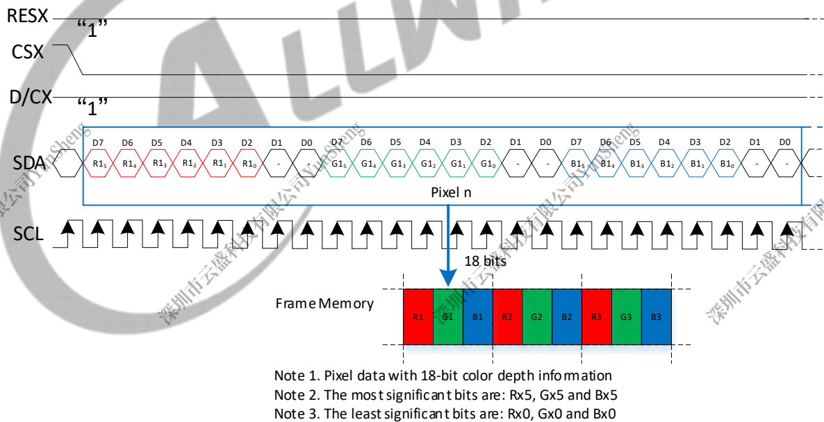
Figure 16-76 RGB666 4-Line Interface Transmit Video Format
