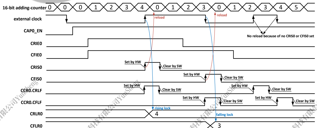
Figure 16-13 PWM0 Channel Capture Timing
