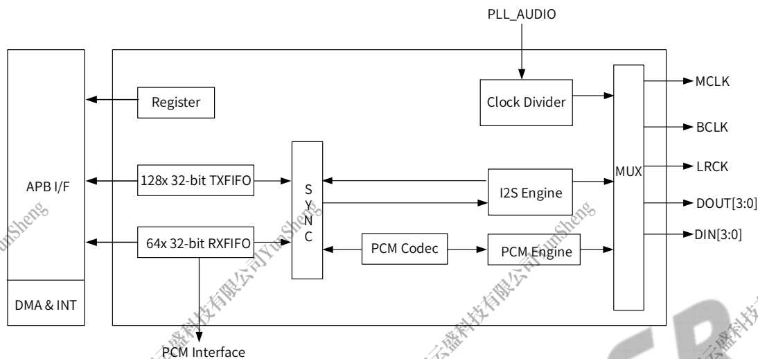
Figure 15-14 I2S/PCM Interface System Block Diagram
