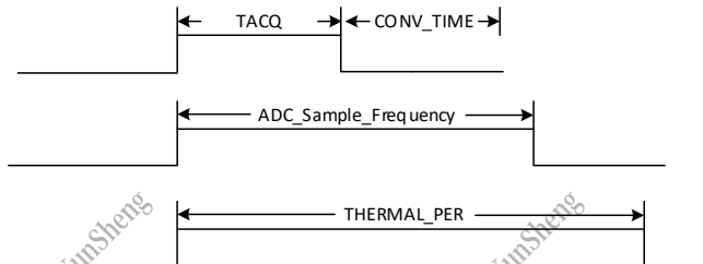
Figure 7-2 Thermal Sensor Timing Requirement
