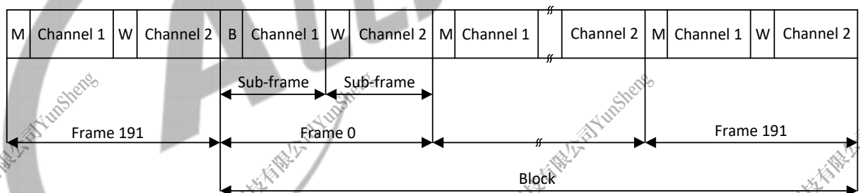
Figure 15-25 OWA Frame/Block Format
