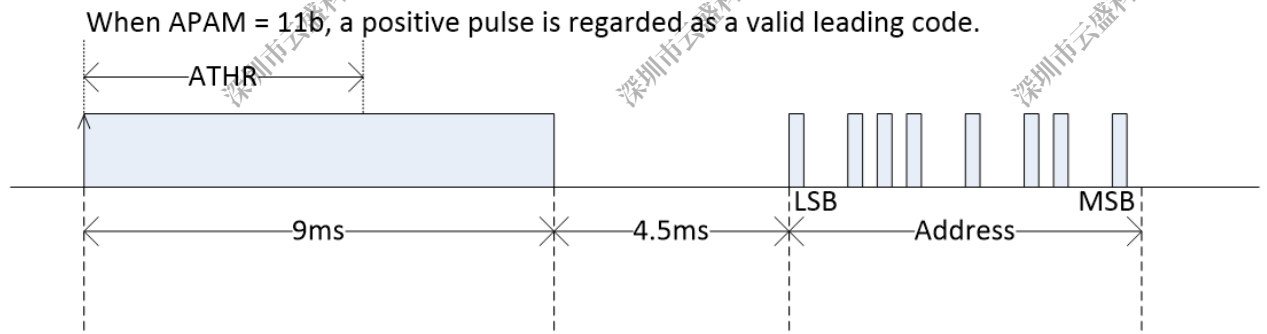
Figure 16-90 APAM Definition
