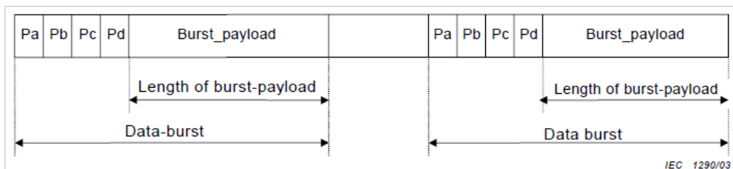
Figure 15-27 Data-burst Preamble
