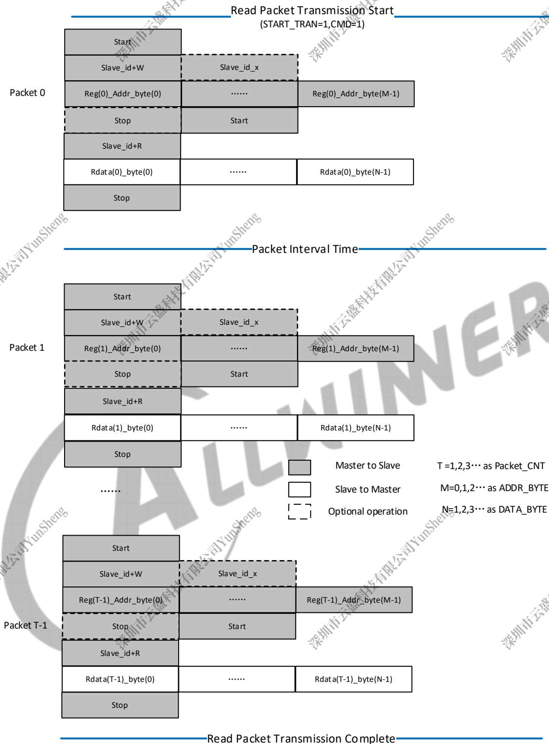
Figure 16-25 TWI Driver Read Packet Transmission
