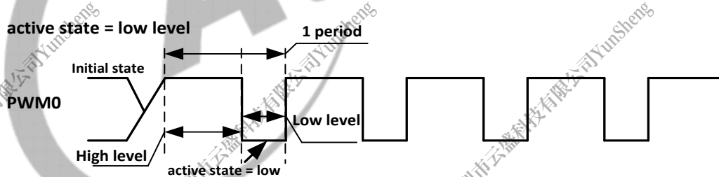
Figure 16-9 PWM0 Low Level Active State
