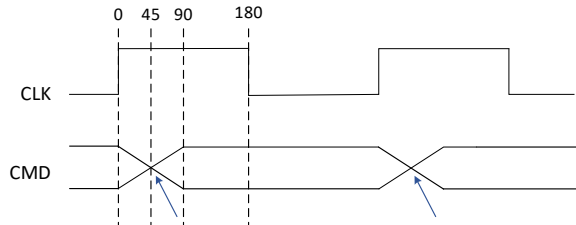
DDR4 (2x mode) Drive Delay = 1
