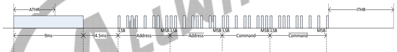
Figure 16-85 A Typical Pulse Train of the NEC
