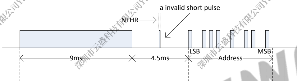
Figure 16-89 NTHR Definition
