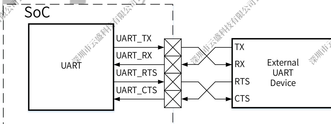
Figure 16-43 Application Diagram for RTS/CTS Auto flow Control
