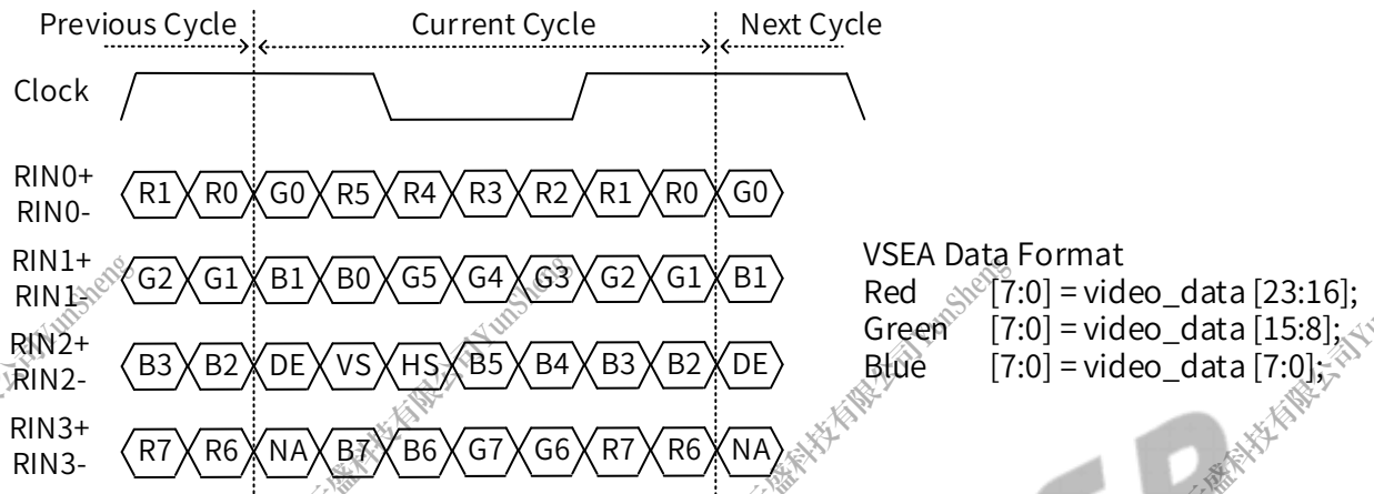
Figure 14-3 Single LVDS VSEA Mode
