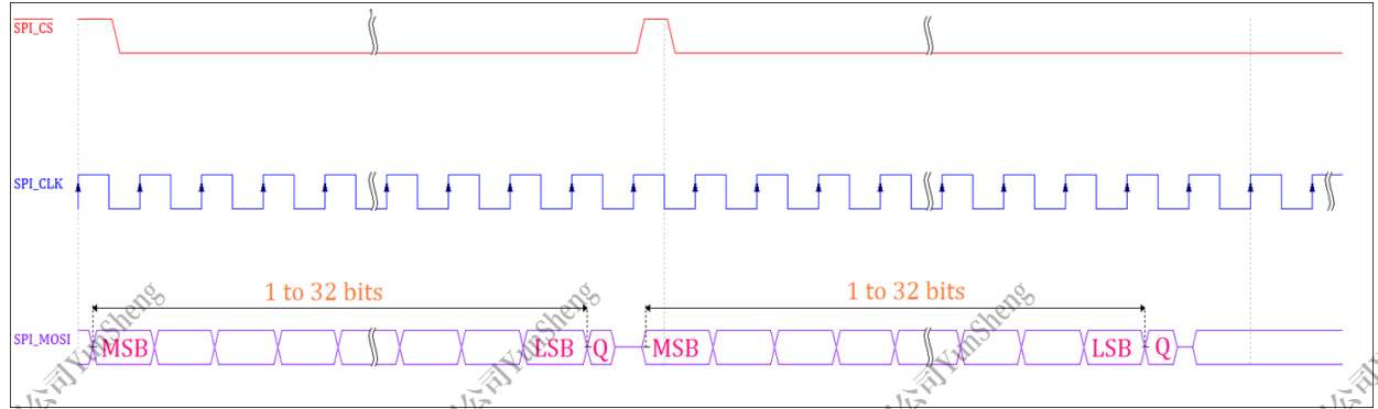
Figure 10-20 SPI 3-Wire Mode
