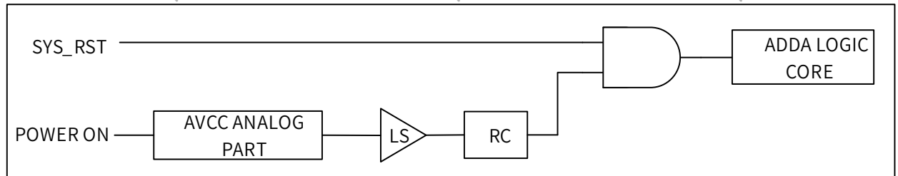
Figure 15-4 Audio Codec Analog Part Reset System
